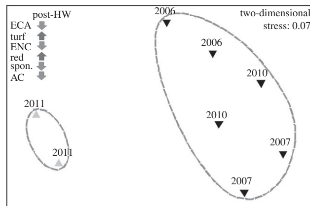
Figure 5. MDS ordination of understorey community structure at JB, before and after the warming event, based on a Bray–Curtis similarity matrix generated from square-root-transformed percentage cover data. Centroids represent understorey community structure at two independent study sites within JB for each survey year (averages of six replicate quadrats per year per site combination). Also shown is the response of key discriminatory taxonomic groups to the HW (i.e. increased or decreased per cent cover) based on SIMPER analysis (see table 3 for results and taxa abbreviations). Grey triangle, post-HW; inverted black triangle, pre-HW.
